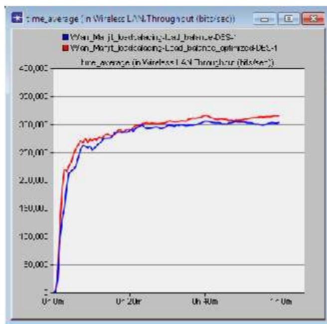
Fig 5: Throughput comparison for both scenarios
