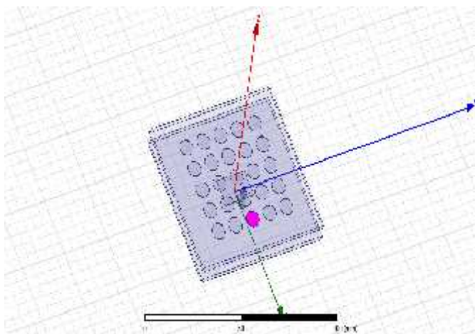
Fig. 2 Patch antenna with EBG structure
