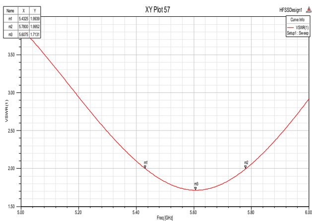
FIG.7 VSWR of Patch antenna with EBG
