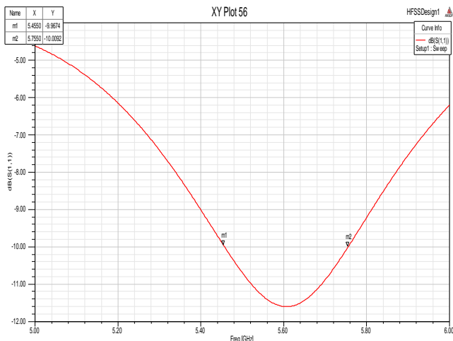
FIG.6 Return loss of Patch antenna with EBG
