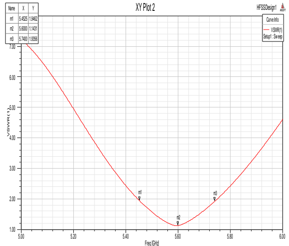
FIG.4 VSWR plot for Patch antenna without EBG
