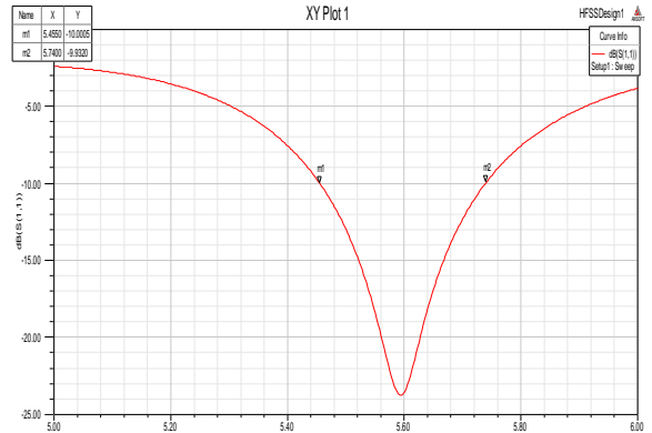
FIG.3 Return Loss of Patch antenna without EBG
