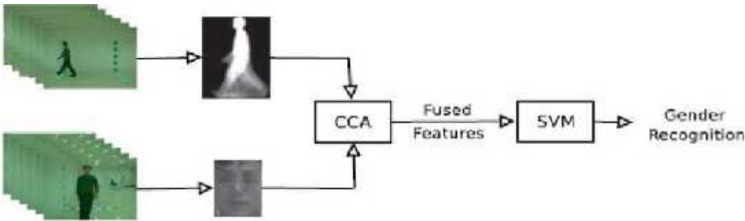
Figure 1: Face-gait fusion for gender (secondary identifier) extraction Using gait for determining gender is a novel approach, and has not been explored before. Most of the existing work attempts to classify gender from human faces. In our work, we would like to investigate structural features and dynamic features of gaits for gender recognition, by adopting Gait Energy Image (GEI), a novel spatiotemporal compact representation of gaits. GEI has been demonstrated to be effective for representing gaits in the human identification problem. Using background subtraction techniques, the walking subjects can be extracted from the original image sequences to derive binary silhouette image sequences. To make the gait representation insensitive to the distance between the camera and the subject, we can perform silhouette preprocessing procedures including size normalization and horizontal alignment. Some examples of normalized and aligned silhouette images are shown in Figure 2. The entire human gait sequence can be divided into cycles as human walking repeats at a stable frequency. We decide the gait cycles by counting the number of foreground pixels in the bottom half of the silhouette and the two
