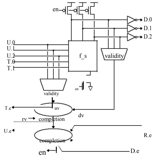
Figure 12. Rproc circuit implementation.
