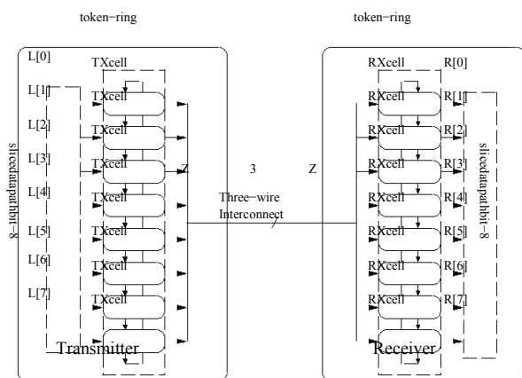
Figure 5. Basic 8:1 multiplexed transceiver architecture.
