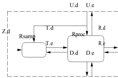
Figure 10. Demultiplexed receive cell (RXcell).
