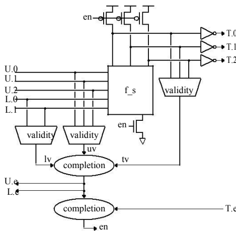
Figure 8. Tproc circuit implementation.
