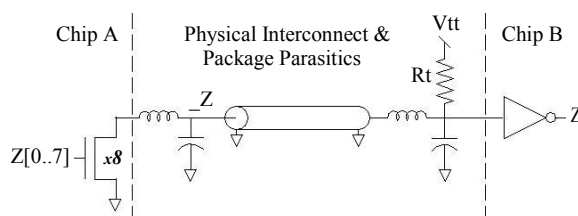
Figure 6. Electrical interconnect configuration.
