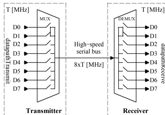
Figure 1. Serial link using multiplexed transceivers.
