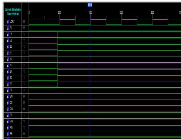
Fig. 6: Simulation results when traffic is equal on all sides
