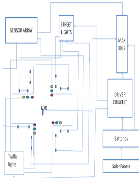
Fig.2: Block diagram of Street light and Traffic controller
