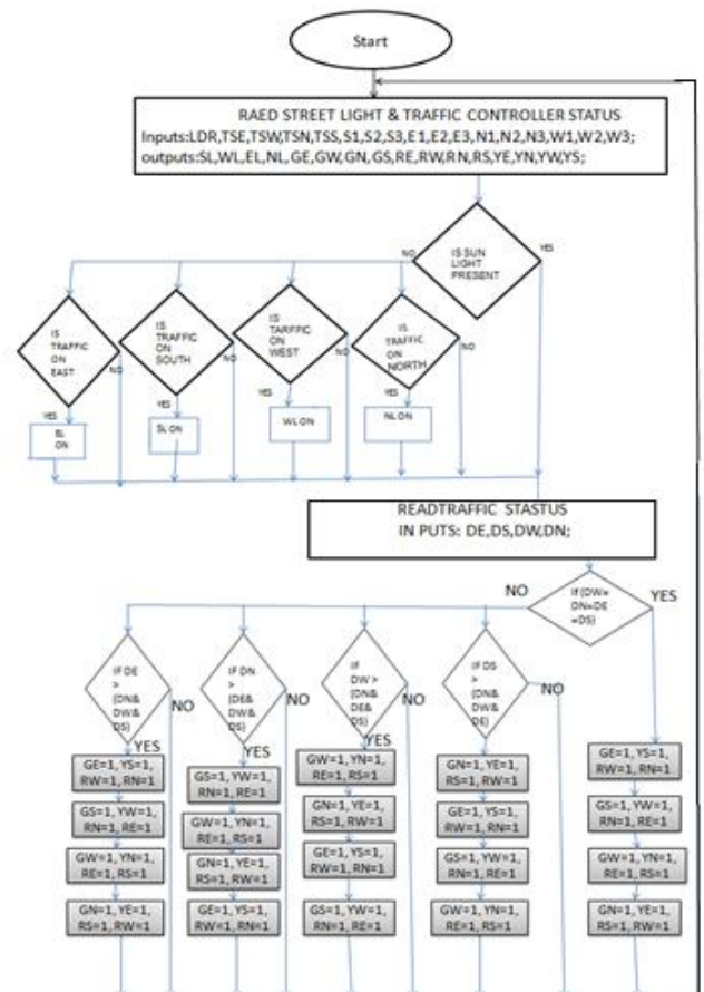
Fig.3: Flow chart of traffic and street light control
