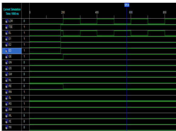
Fig. 4: Simulation results when more traffic on East
