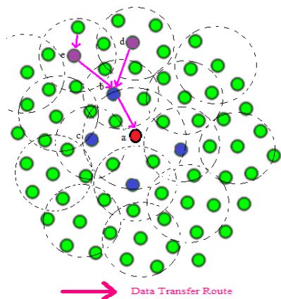
Fig.6 Data transfer route of sensor nodes
