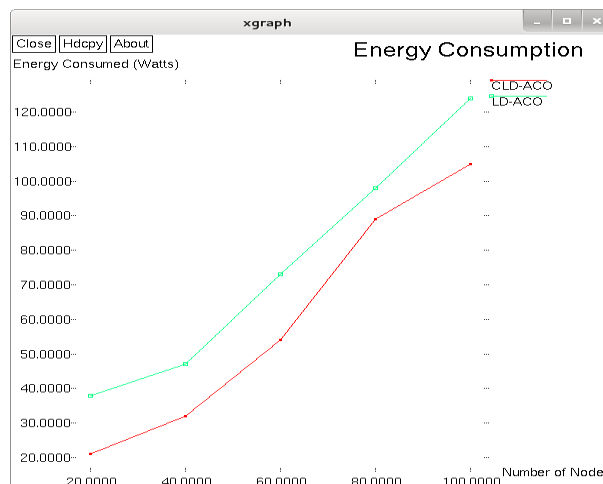
Fig.7 Nodes vs. Energy Consumption
