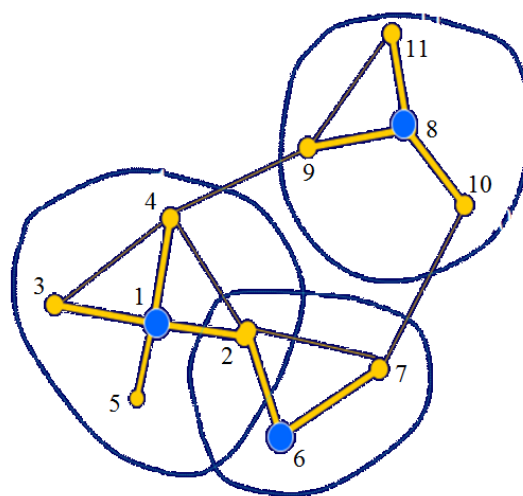
Fig.3 Cluster Formation
