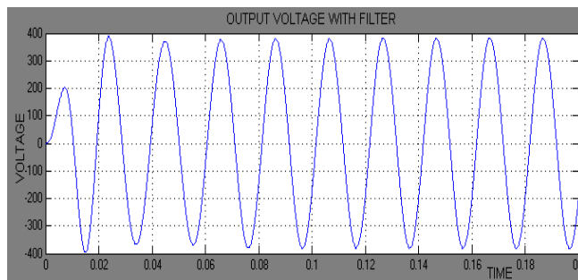
Fig.16. Output voltage of inverter with filter
