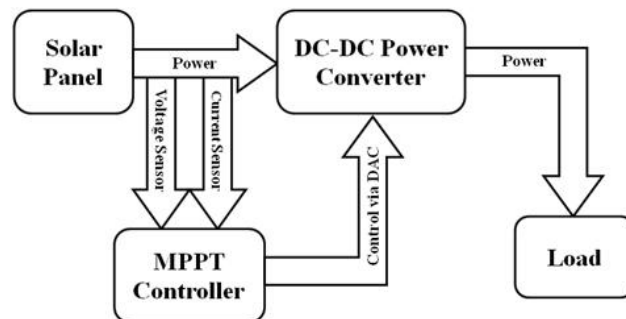
fig 5.MPPT in PV system.
