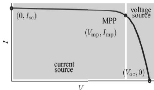
Fig. 4. I-V Characteristic of Practical PV Module
