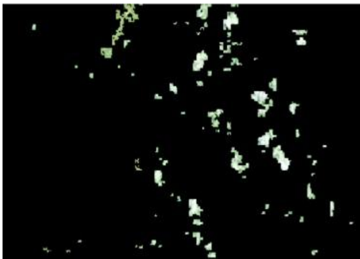
Fig. 3 Cloud detection
