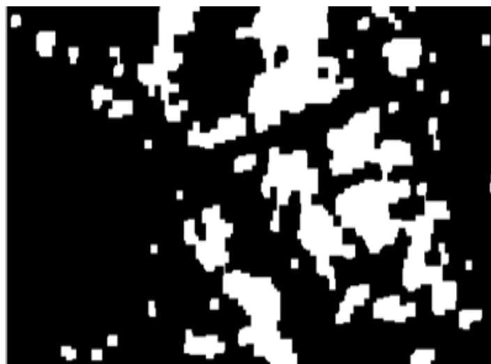
Fig.4 Blob detection
