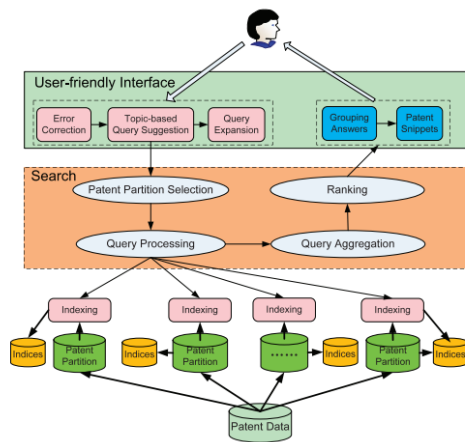
Fig. 1. User-friendly patent search architecture.
