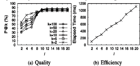
Fig. 2. Effect on \ell .
