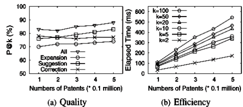
Fig. 4. Scalability.
