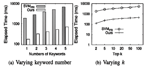
Fig. 3. Efficiency comparison.
