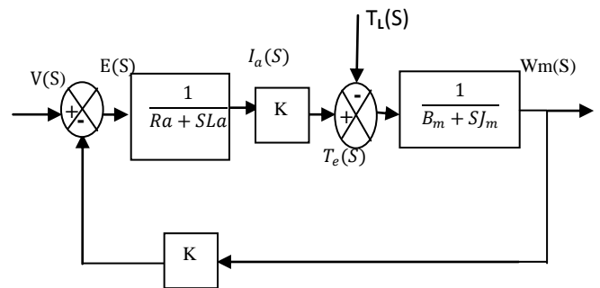
Fig.6 Block diagram of the DC motor
