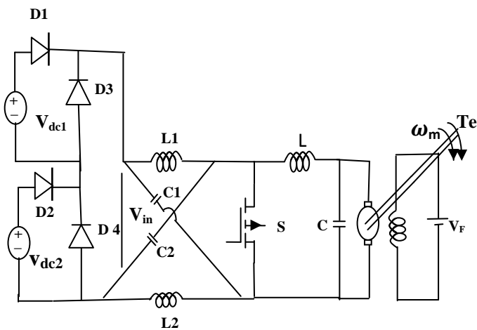
Fig1.DC Motor fed with double input Z-source DC-DC converter
