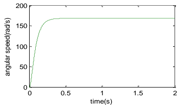
Fig15. angular speed of the dc motor state 3
