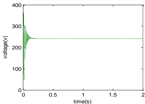
Fig7. Double input DC-DC converter output voltage in state 1
