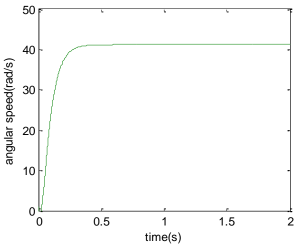
Fig12. angular speed of the dc motor in state 2
