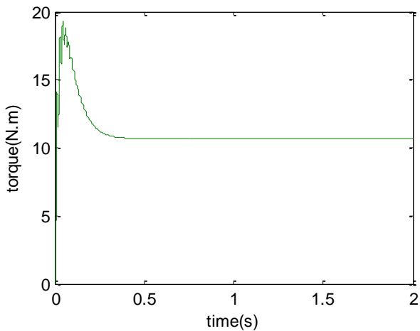
Fig11. electromagnetic torque in state 2
