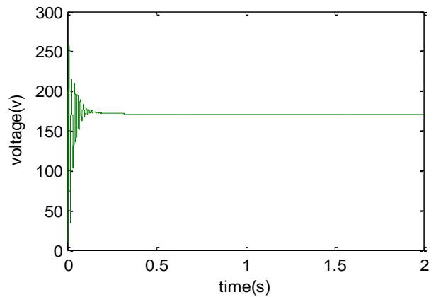
Fig13. converter output voltage in state 3
