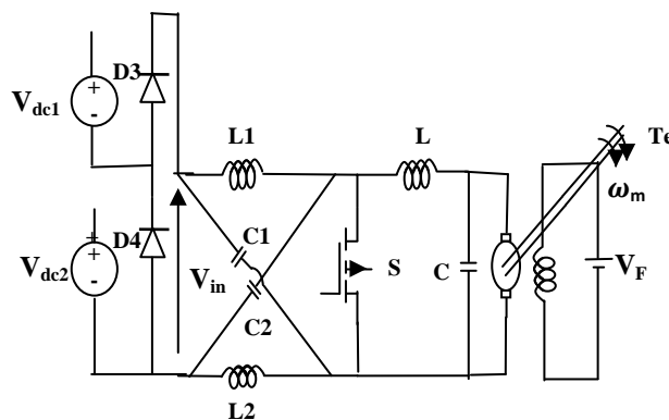
Fig5. Double input DC-DC converter state4 equivalent circuit
