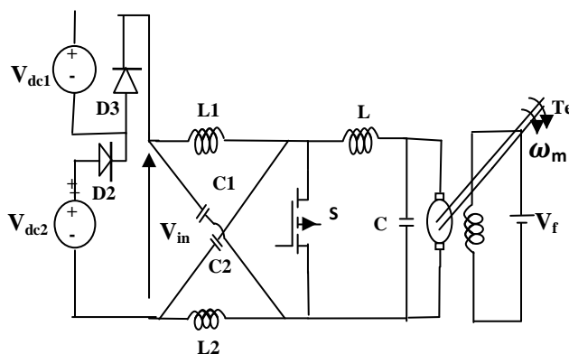
Fig4. Double input DC-DC converter state3 equivalent circuit
