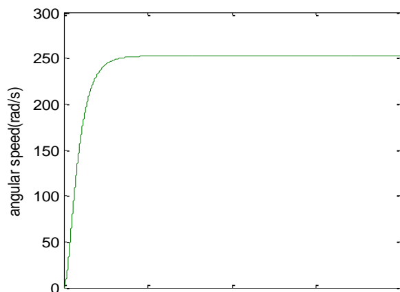
Fig9. Angular speed of the dc motor
