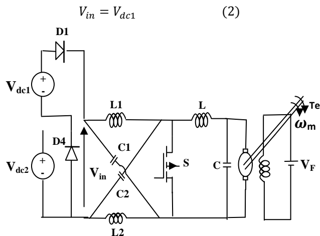
Fig3. Double input DC-DC converter state2 equivalent circuit
