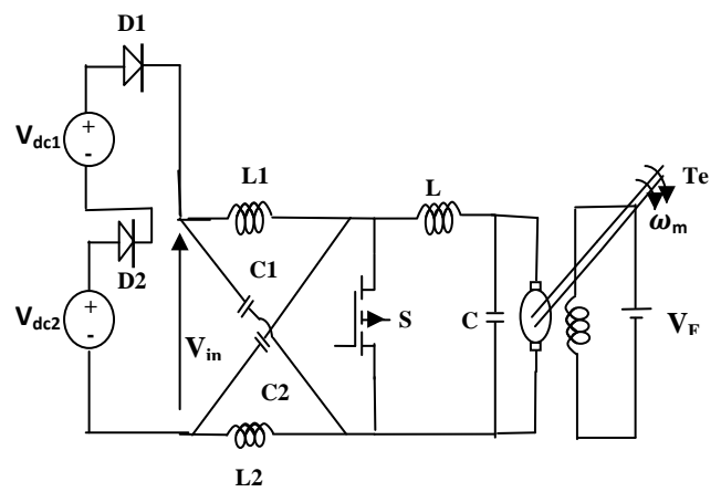
Fig2. Double input DC-DC converter state1 equivalent circuit
