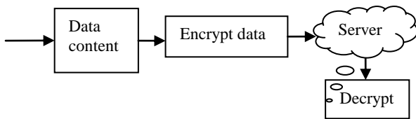
(Blowfish algorithm)
