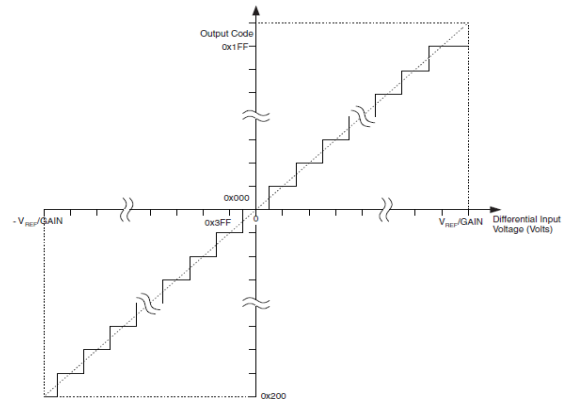
Fig 2. Differential Measurement Range
