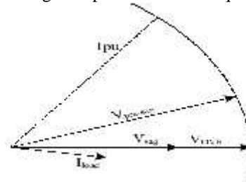
In-Phase Compensation Techniques
