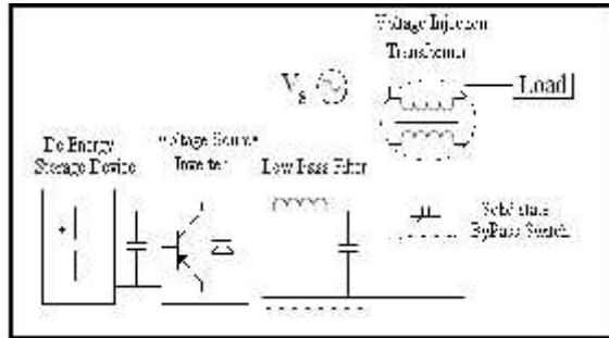
DVR Power circuit
