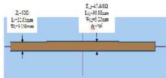
Figure 4.3 Simulated design of transmission lines
