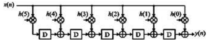
Fig.2. DFG 2 of transposed form structure for N=6.For output y(n)
