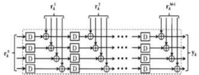
Fig.11. Internal structure of Pipelined Adder Unit (PAU)
