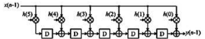
Fig.3. DFG 3 of transposed form structure for N=6.For output y(n-1)
