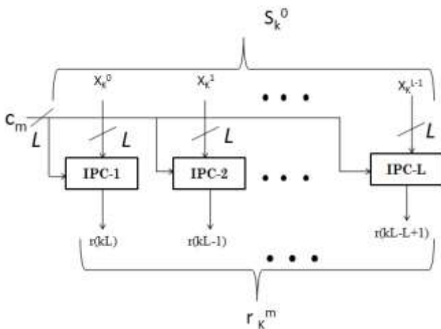
Fig.9. Internal structure of (m + 1)_{th} IPU.
