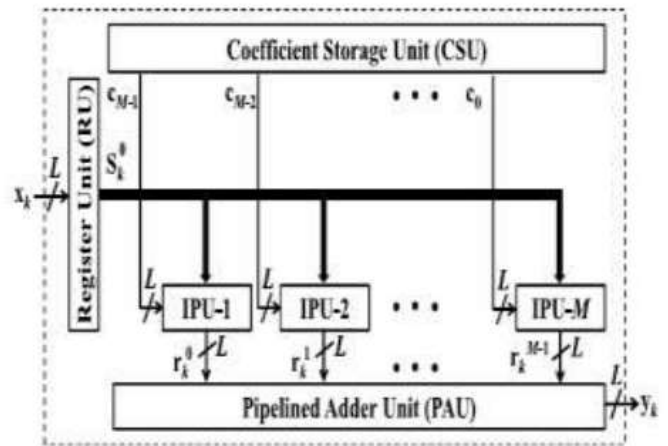
Fig.7. Block of reconfigurable coefficient FIR filter (L,M).
