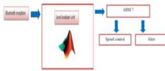
Fig.3 Receiver Block
