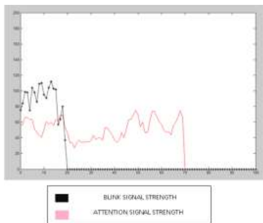
Fig.3 MATLAB Output
