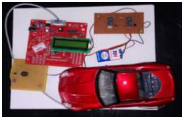
Fig. 5 Hardware Setup
