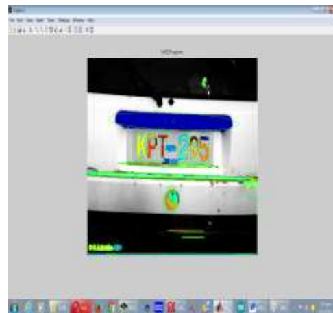
Fig.3. Original Image
