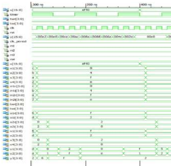
Figure 7 : simulation of the proposed work OFDM-BERT
