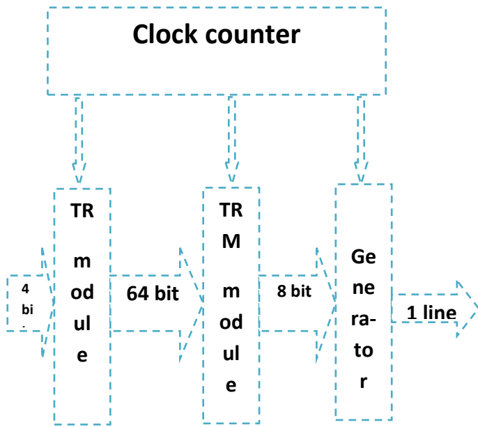
Figure 5 Proposed QPSK Modulator
