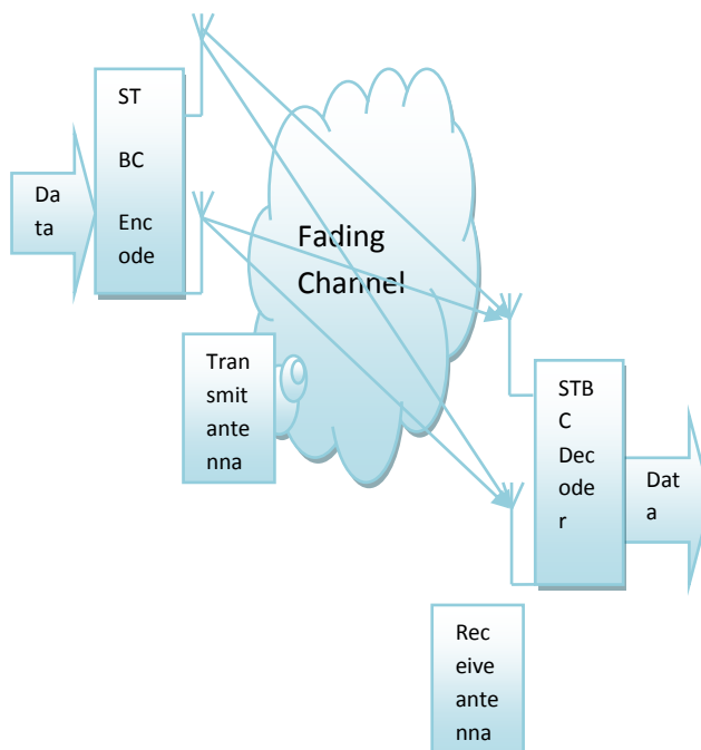
Fig 2 A typical communication system utilizing space-time coding
