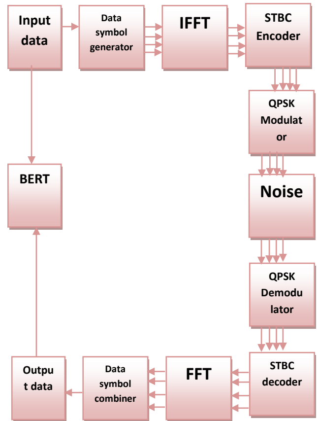
Figure 1 OFDM system
