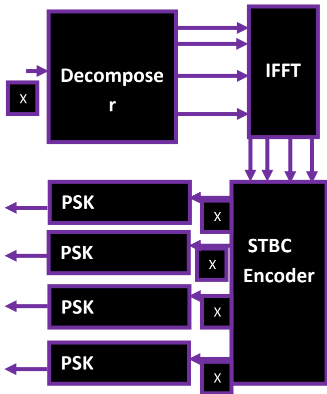
Figure 4 Proposed OFDM transmitter
