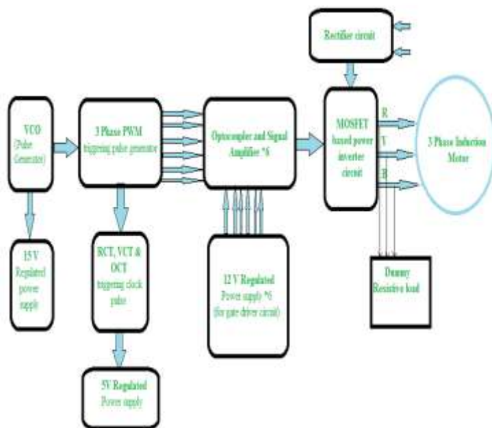
Fig. 1. Multilevel inverter based block diagram
