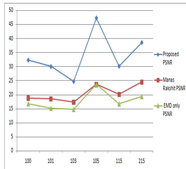
Figure 6 PSNR comparison without external noise in MIT-BIH database
