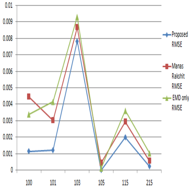
Figure 7 RMSE comparisons without external noise in MIT-BIH database
