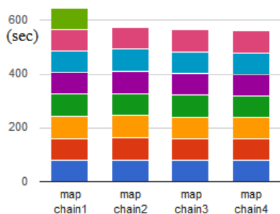
Figure 3.4: Map wave of WordCount.
