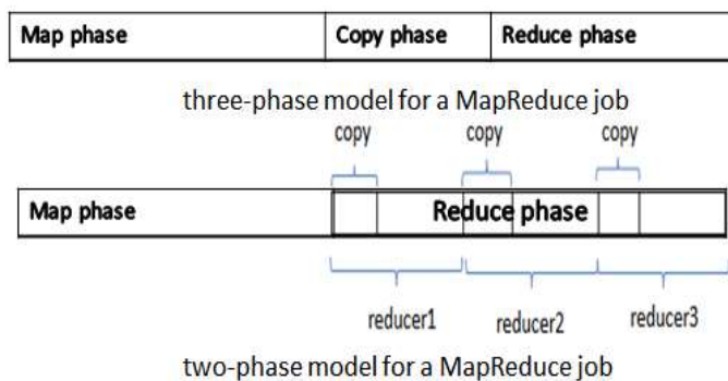
Figure 3.2: Models to describe a MapReduce job
