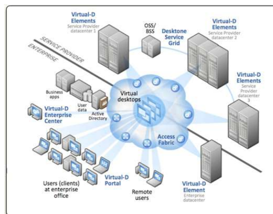
Figure 1.cloud computing environment
