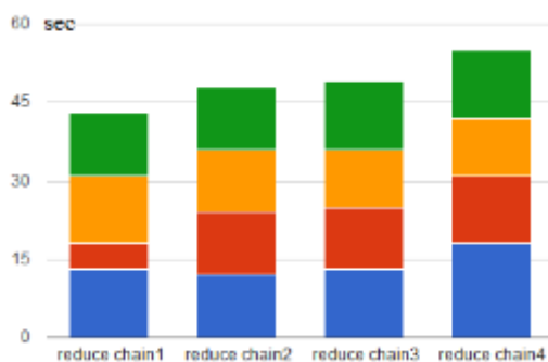
Figure 3.5: Reduce wave of WordCount.
