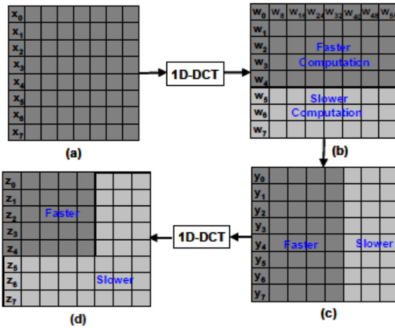
Fig. 3: Input image matrix and DCT matrices after 1 st and 2 nd transform.
