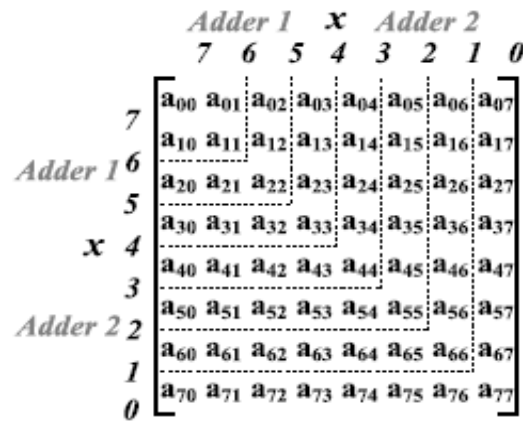
Fig. 4: Partitioning of the input matrix.
