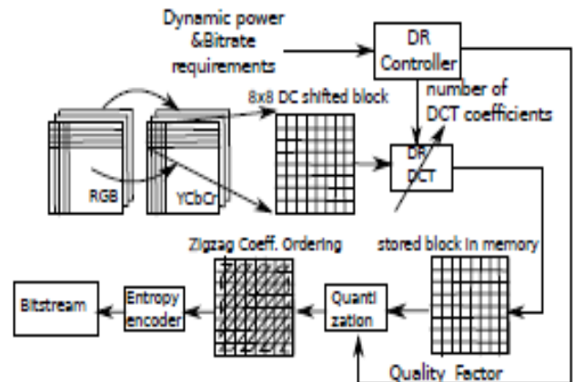
Fig. 5: Dynamic reconfigurable DCT architecture
