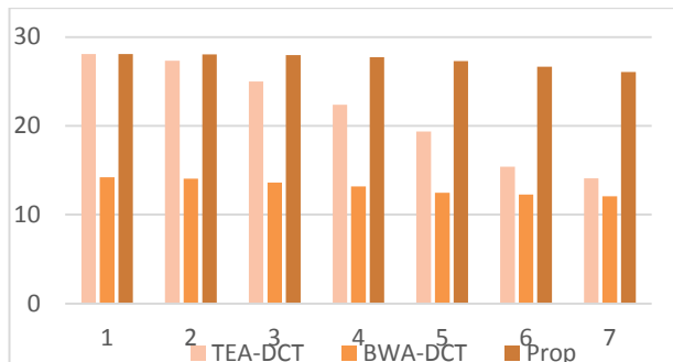
Fig. 10: PSNR of various DCT for varying ET
