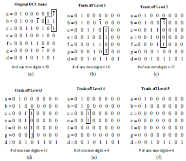
Fig. 2: Constant multiplier approximation
