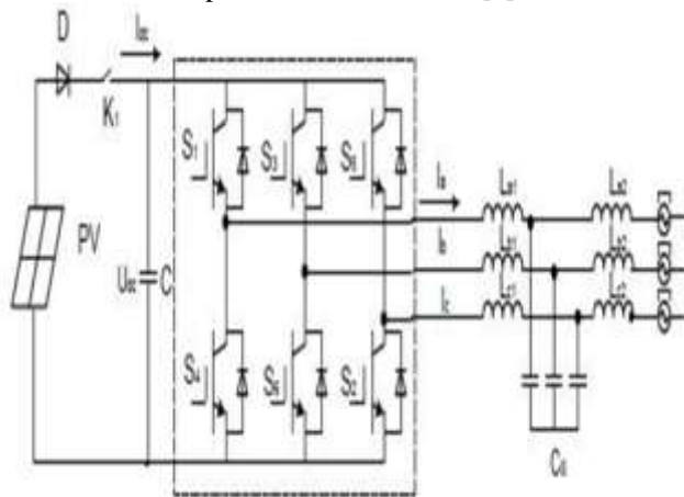
Fig.1. Topological structure of three-phase PV grid-connected inverters with LCL filter.
