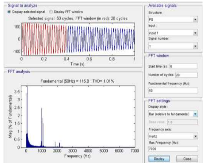
Fig. 14. THD of the proposed system is 1.01%.
