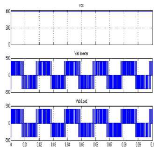
Fig.7. Input voltage and Load voltage waveform.
