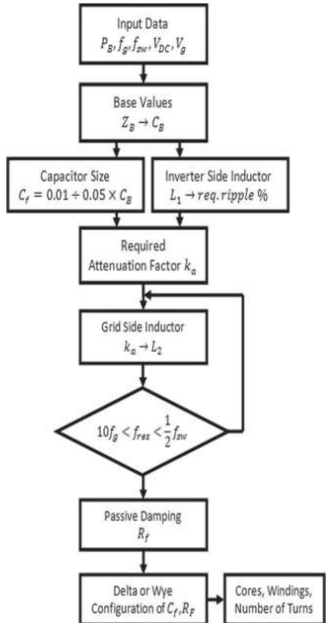
Fig. 4. LCL filter design algorithm.
