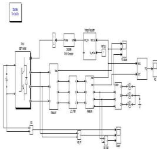
Fig.11. Closed loop circuit of grid connected system.
