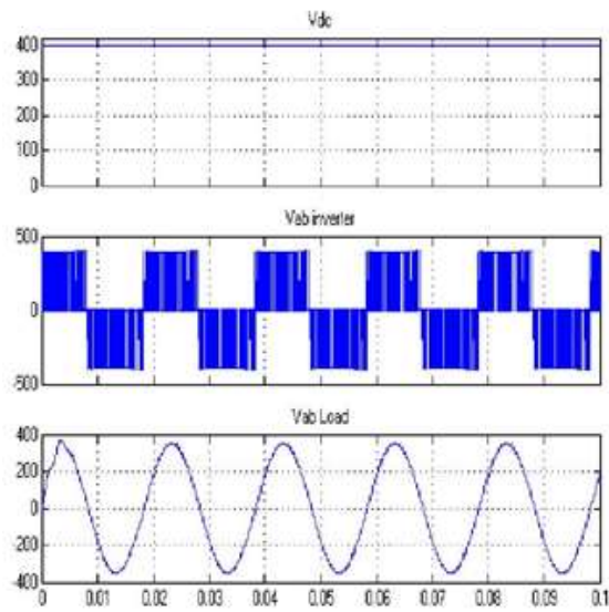
Fig.10. Comparison of three voltages.
