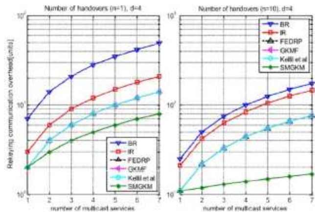
Fig. 10. Pairwise rekeying communication overheads.
