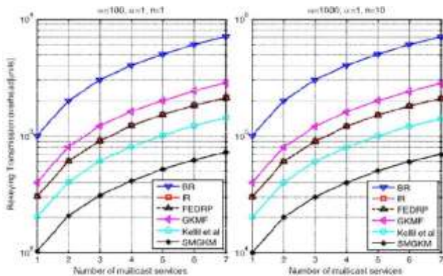
Fig. 9. Rekeying Transmission overhead.
