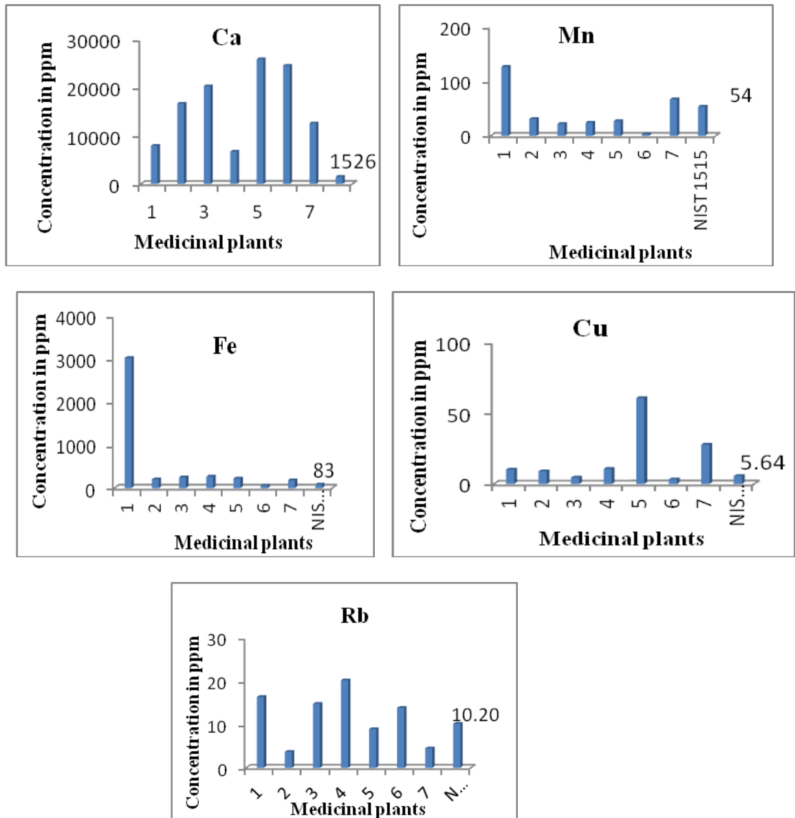
Figure 2. Graph of S, K, Ca, Mn, Fe, Cu and Rb concentrations in studied plant samples with NIST 1515 standard.
