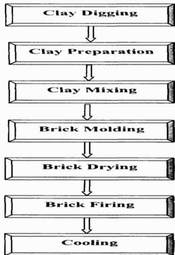
Figure 1.1: Flow Diagram For Brick Manufacturing
