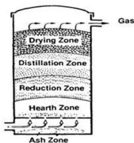
Fig.2. Updraft gasifier [4]
