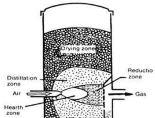
Fig.4. Cross-draft gasifier [5]
