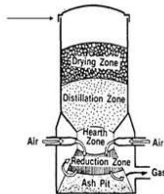
Fig.3. Downdraft gasifier [4]
