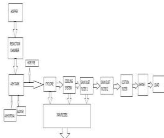
Fig-5 Downdraft Gasifier
